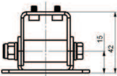
Mounting base with protective housing
